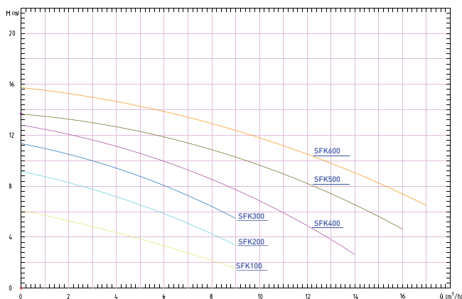
Pump flow head curve
